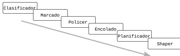
FIGURA 17.10: Pipeline QoS
